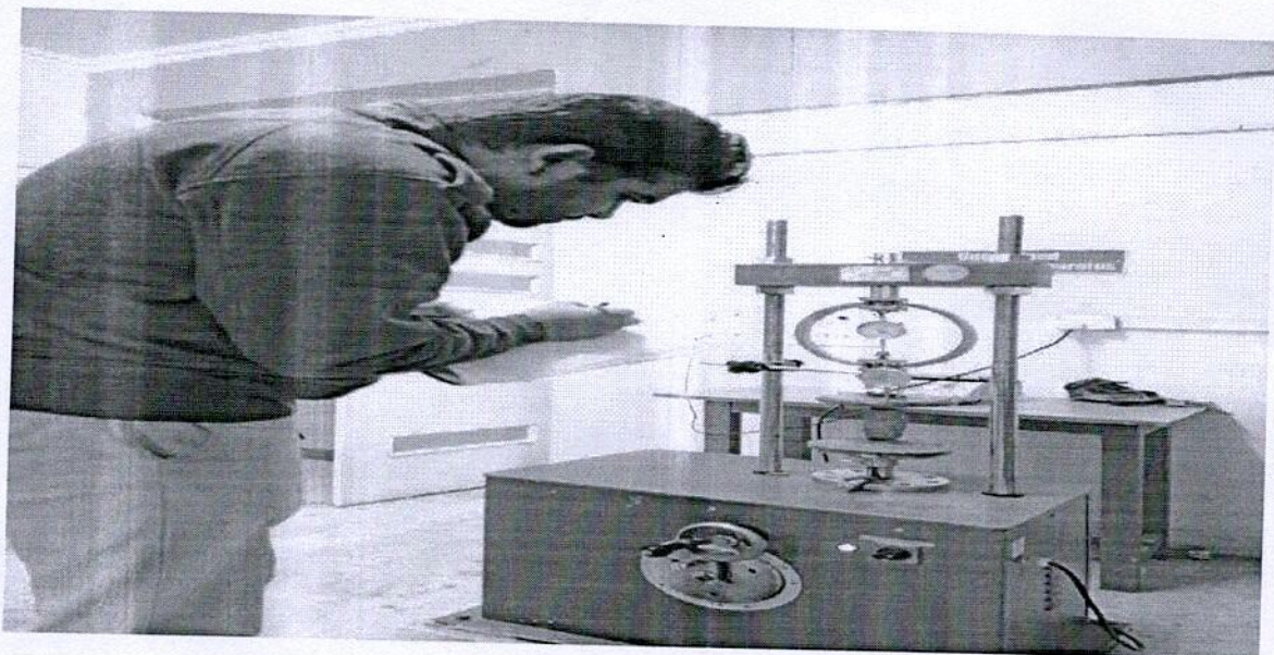
Unconfined Compression test on given soil sample
