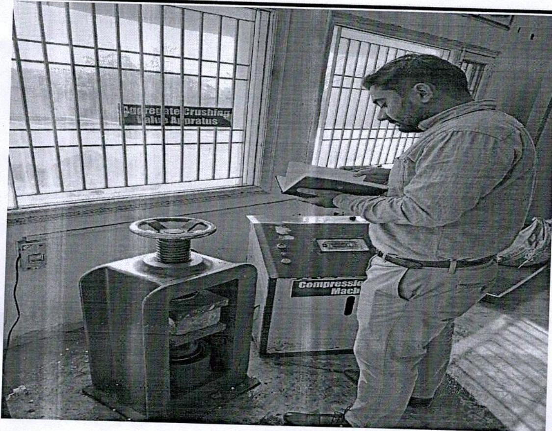
Compression testing on given concrete block sample
